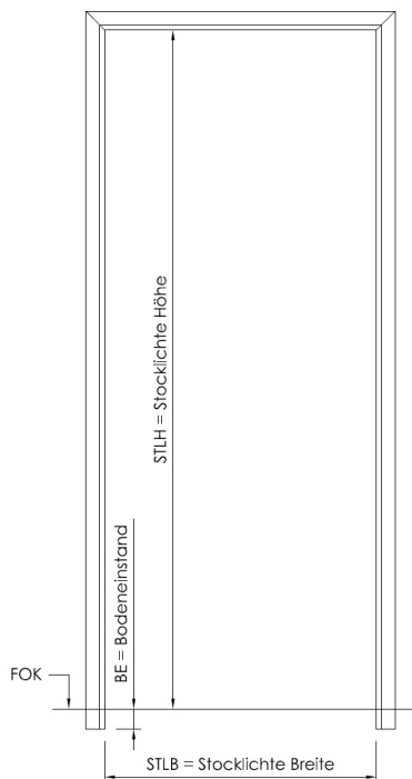
Pendeltürzarge
